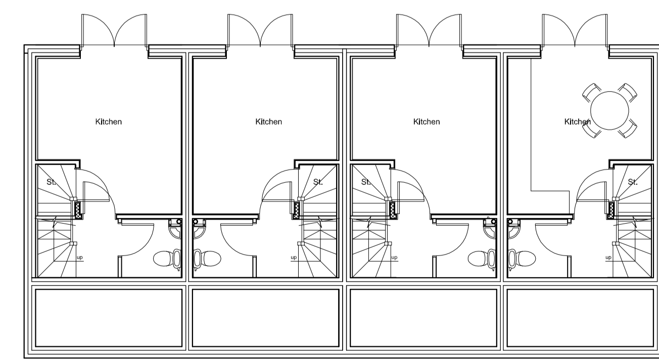
Lower Ground Floor Plan 1:100
